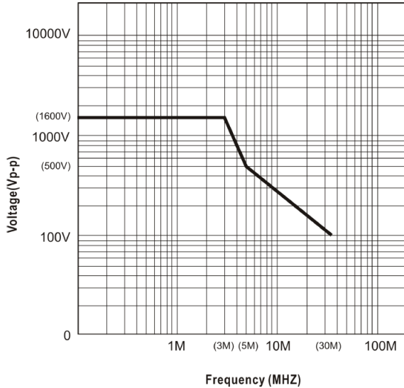
Figure 1 CT4068-NA Derating Curve
