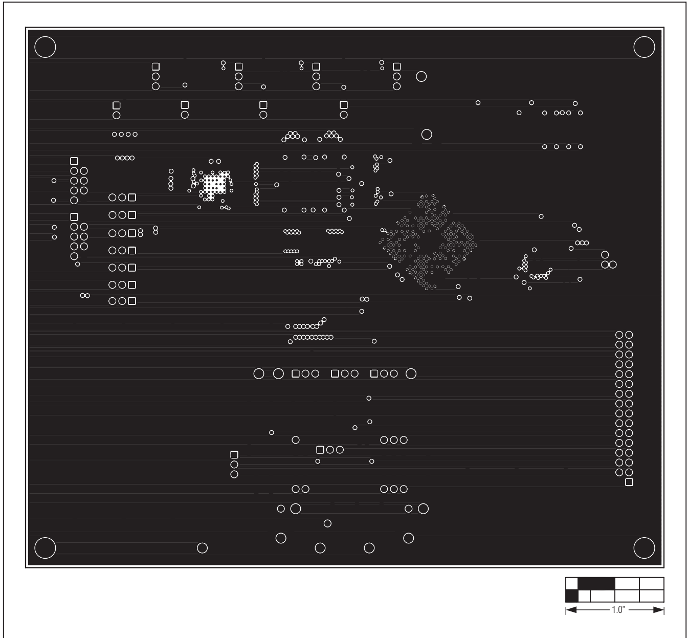
Figure 9. MAX1105 EV Kit PCB Layout—Layer 2
