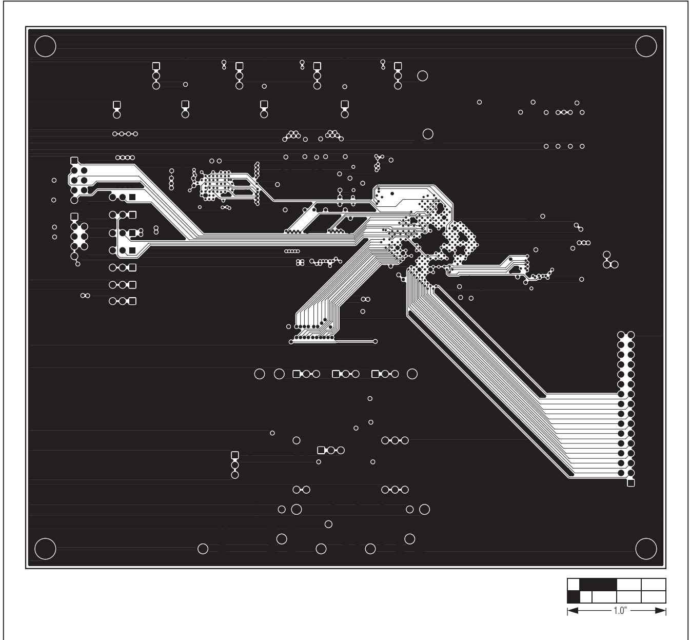
Figure 10. MAX11105 EV Kit PCB Layout—Layer 3
