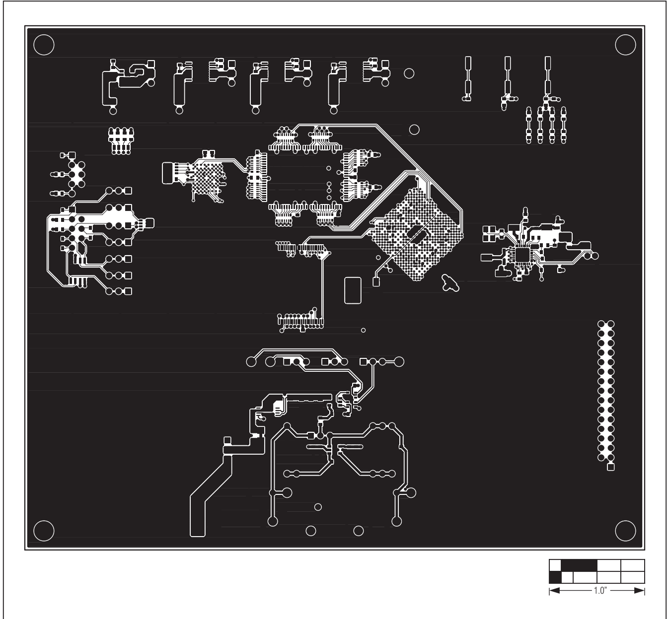
Figure 8. MAX11105 EV Kit PCB Layout—Component Side
