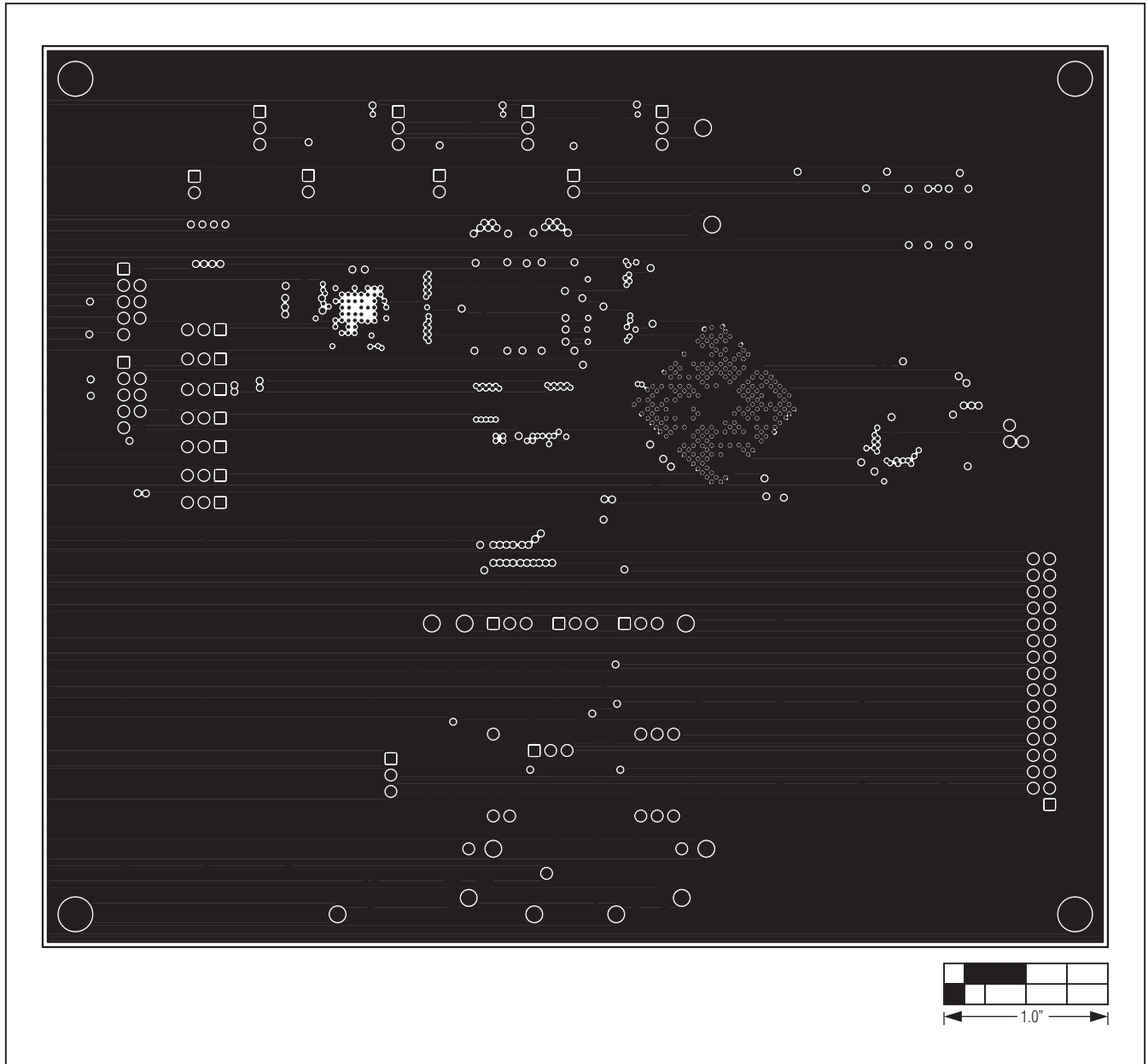
Figure 15. MAX1105 EV Kit PCB Layout—Layer 8
