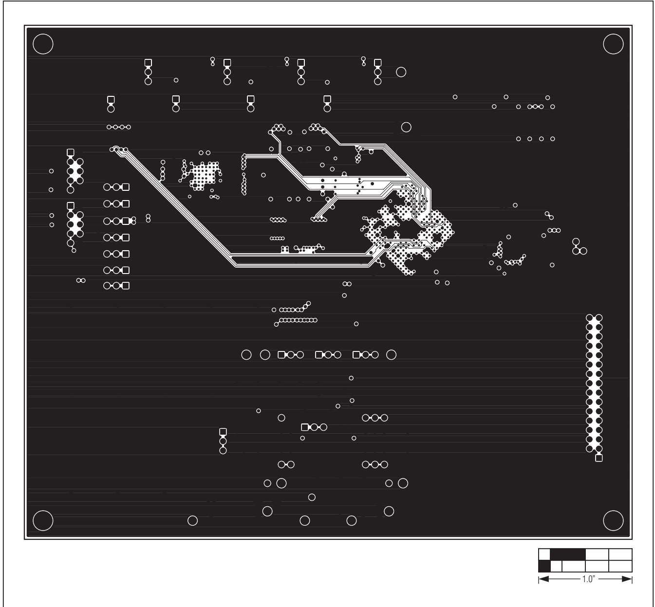
Figure 16. MAX11105 EV Kit PCB Layout—Layer 9
