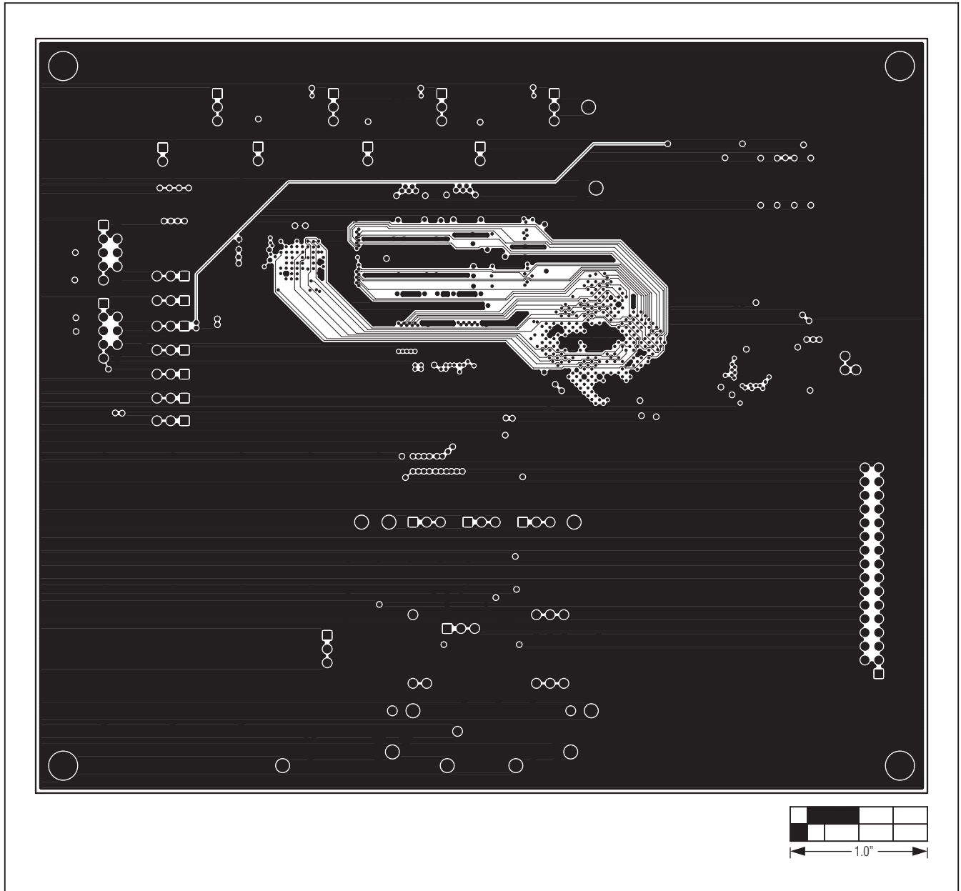
Figure 13. MAX11105 EV Kit PCB Layout—Layer 6
