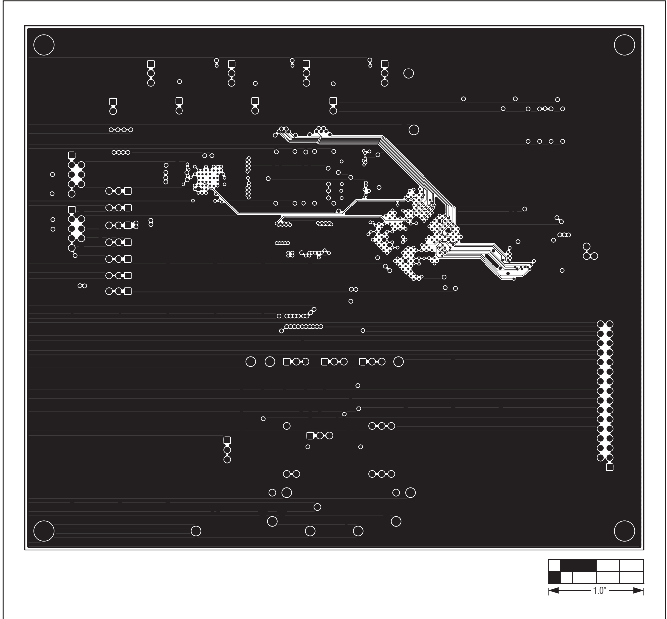
Figure 14. MAX11105 EV Kit PCB Layout—Layer 7
