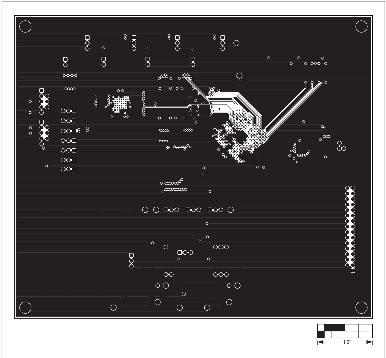
Figure 11. MAX11105 EV Kit PCB Layout—Layer 4
