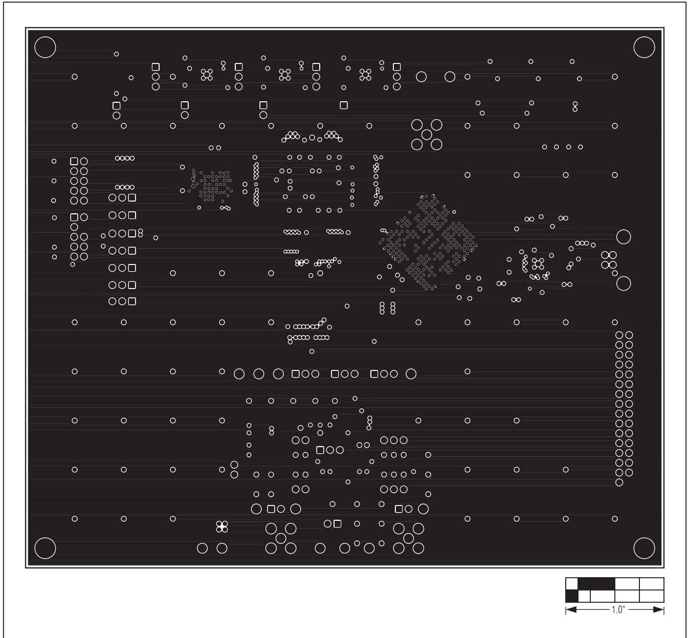
Figure 18. MAX11105 EV Kit PCB Layout—Layer 11
