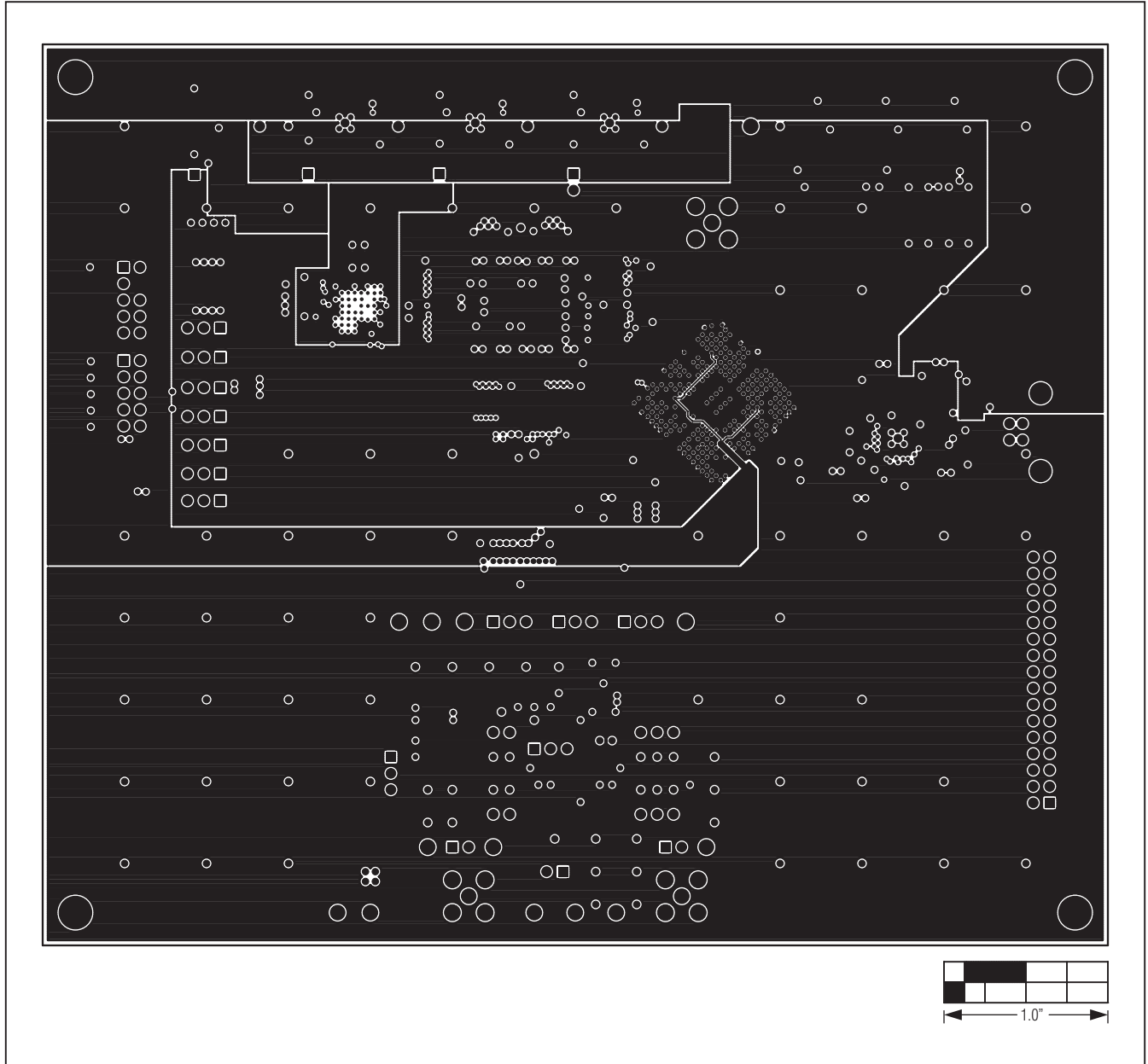
Figure 12. MAX11105 EV Kit PCB Layout—Layer 5
