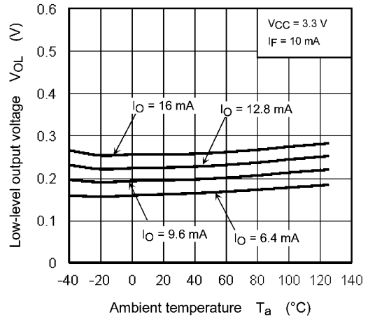
Fig. 12.2.4 V_{OL} - T_a
