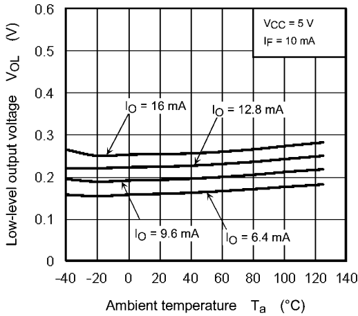
Fig. 12.2.3 V_{OL} - T_a
