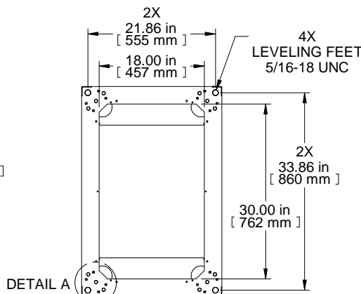
BOTTOM VIEW BOTTOM OPENING
