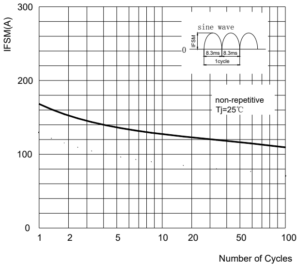
Figure1 Surge Forward Current Capability
