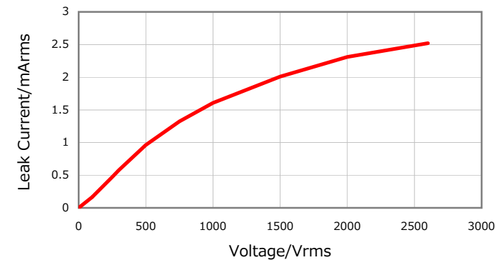
Leak Current
